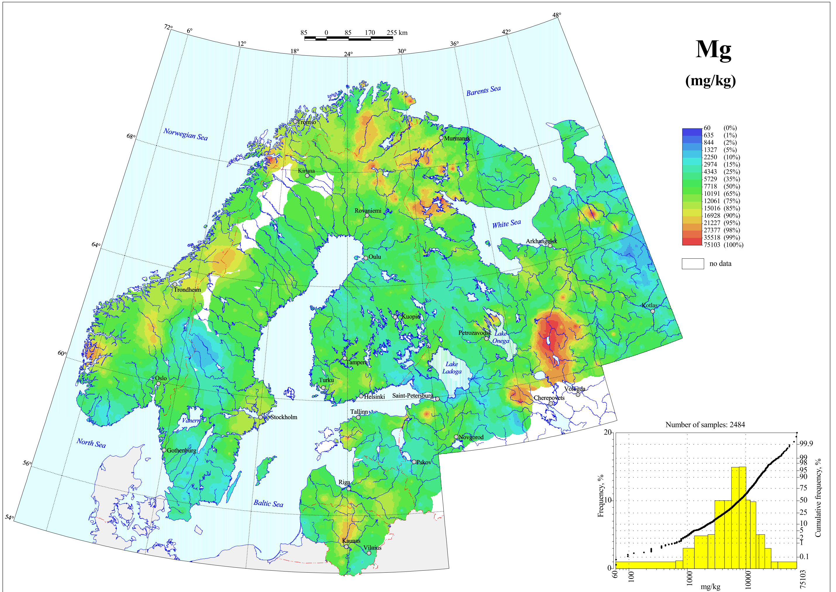
Magnesium in C-horizon, Grain Size <2 mm, Total Content
